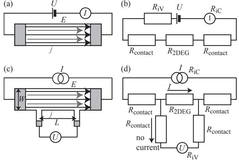
Fig. 10.8 (a) Two-terminal measurement with a bar geometry. (b) Equivalent circuit with contact resistances R_{\text{contact}} and the internal resistances of the voltage source R_{iV} (typically < 50\Omega ) and of the ammeter R_{iC} (typically \leq 10\Omega ). (c) Four-terminal measurement with a bar geometry. (d) Equivalent circuit with contact resistances R_{\text{contact}} , the internal resistance of the voltmeter R_{iV} (typically > 10\text{M}\Omega ) and the internal resistance of the current source (typically > 10\text{M}\Omega ).
