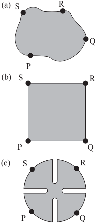
Fig. 10.16 Sample geometries for the van der Pauw method. (a) arbitrary shape (b) square shape (c) 4-foliate sample shape.
