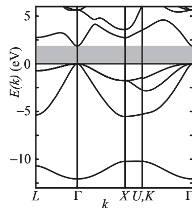
Fig. 3.4 Result of local pseudopotential calculations for GaAs. Spin-orbit interaction effects were neglected. The fundamental band gap is shaded in gray.
