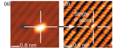
Fig. 4.2 STM images of atomically controlled single phosphor atom incorporation into Si(001). (a) Hydrogen terminated Si(001) surface with a hydrogen desorption point. (b) The same area after \text{PH}_3 dosing and annealing showing a single P atom incorporated at the location defined by the H-desorption point. (Reprinted with permission from Schofield, 2003. Copyright 2003 by the American Physical Society.)
