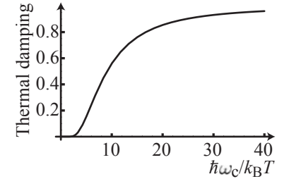
Fig. 16.14 Temperature-dependent factor 2\pi^2 k_B T / \hbar\omega_c \sinh[2\pi^2 k_B T / \hbar\omega_c] plotted versus \hbar\omega_c / (k_B T) .
