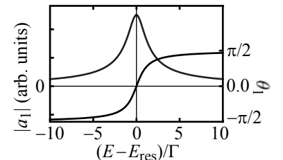
Fig. 21.10 Calculated magnitude and phase of the resonant transmission through a single energy level in the Lorentz approximation.
