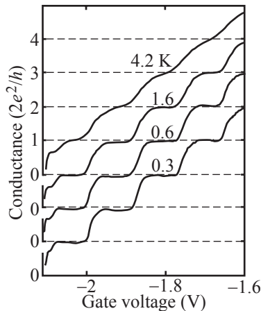
Fig. 11.5 Experimentally observed temperature dependence of the conductance quantization in a quantum point contact. (Reprinted with permission from van Wees et al. , 1991. Copyright 1991 by the American Physical Society.)
