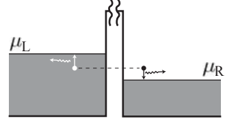
Fig. 11.6 Energy dissipated by a single electron that travels without scattering from source to drain contact through the wire. The wire itself, located between the two reservoirs, is omitted in the drawing for clarity.
