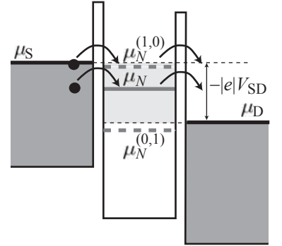
Fig. 18.13 Schematic representation of a quantum dot at finite source-drain voltage. In addition to the ground state transition \mu_N , two excited state transitions are indicated as dashed lines. The upper one, \mu_N^{(1,0)} is in the transport window and therefore contributes to electron transport through the dot.
