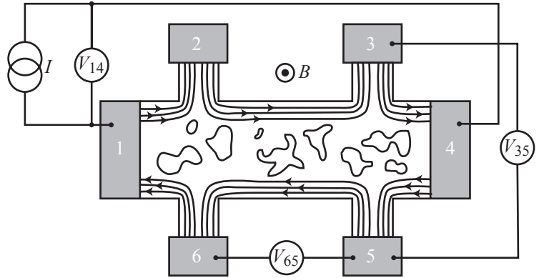
Fig. 16.24 Basic setting which allows the description of the quantum Hall effect in the framework of the Landauer–Büttiker formalism. Quantum Hall edge channels play the role of one-dimensional chiral modes connecting neighboring ohmic contacts. States in the interior of the Hall bar are localized. At integer filling factors, edge channels at opposite edges travelling in opposite directions are completely decoupled. The measurement configurations for two-terminal measurements along the entire Hall bar, and for four-terminal measurements of the longitudinal and the transverse resistance are indicated.
