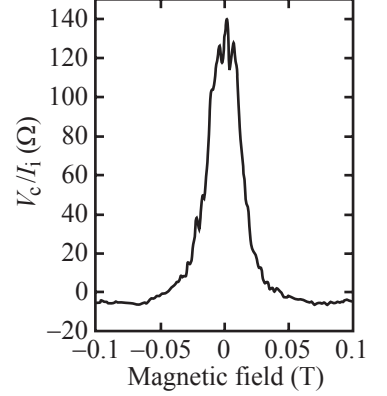
Fig. 13.6 Result of a magnetic steering experiment. Plotted is the nonlocal resistance V_c/I_i . (Reprinted with permission from Molenkamp et al. , 1990. Copyright 1990 by the American Physical Society.)
