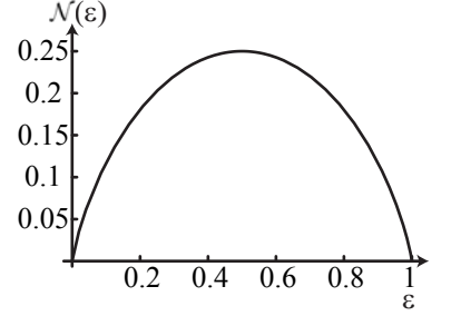
Fig. 22.6 Noise \mathcal{N}(\epsilon) of the AND gate with noise parameter \epsilon .
