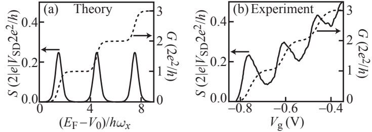
Fig. 20.11 (a) Shot noise calculated for a quantum point contact (solid line) in comparison to the conductance (dashed). For the calculation, the saddle potential model with \omega_y = 3\omega_x was used. (De Jong and Beenakker, 1997. With kind permission of Springer Science and Business Media.) (b) Measured shot noise of a quantum point contact (solid line) in comparison to the measured conductance (dashed) at a temperature of T = 0.4 K. Courtesy of M. Reznikov and M. Heiblum, data similar to Reznikov et al. , 1995.
