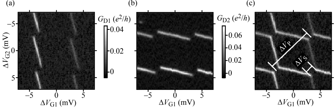
Fig. 19.5 Transport measurements through the two parallel quantum dots shown in Fig. 19.3 which are only capacitively coupled. (a) Conductance resonances in dot 1 as a function of the two plunger gate voltages. (b) Conductance resonances in dot 2 as a function of the same plunger gate voltages. (c) Superposition of the two measurements (a) and (b) resulting in the hexagon pattern of the capacitance model. (Reprinted from Chan et al. , 2003 with permission from Elsevier.)
