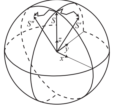
Fig. 15.12 Spin diffusion on the Bloch sphere. (Reprinted from Bergmann, 1982 with permission from Elsevier.)
