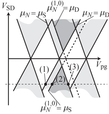
Fig. 18.14 Schematic Coulomb blockade diamonds with an excited state. Current can flow in the light gray triangular shaped regions. Black lines indicate alignment between one of the electrochemical potentials in the leads ( \mu_S or \mu_D ) with a transition \mu_N^{(n,m)} in the dot. The points labeled (1)–(3) refer to the three current steps introduced in the text.
