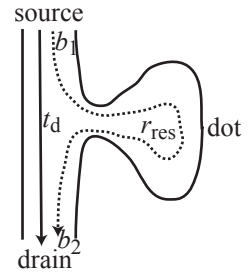
Fig. 21.4 Schematic illustration showing the interference of two alternative paths: the direct transmission with amplitude t_d and the resonant transmission with amplitude b_1 r_{\text{res}} b_2 .
