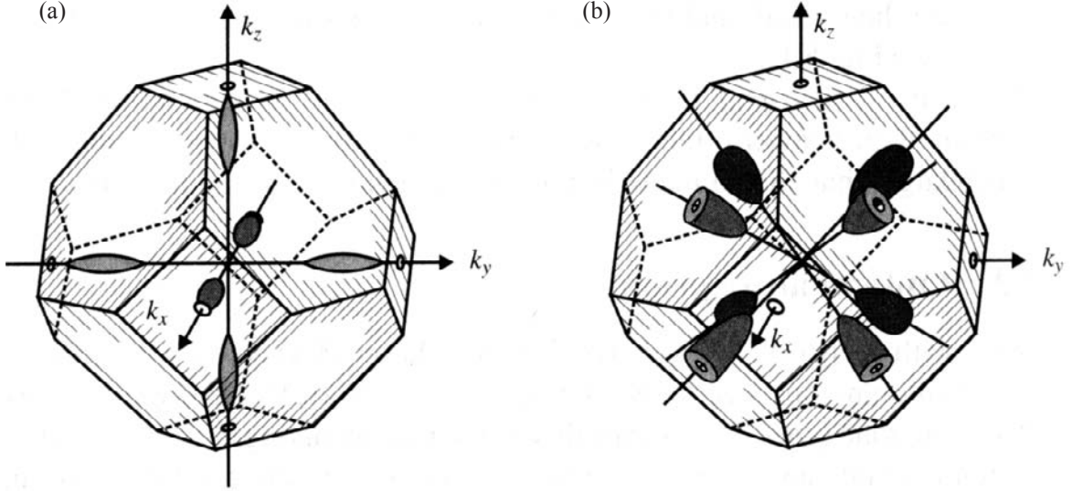
Fig. 3.14 (a) Surfaces of constant energy close to the minima of the conduction band of silicon. (b) Surfaces of constant energy close to the conduction band of germanium (Singleton, 2001).
