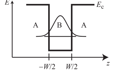
Fig. 5.5 Conduction band edge of an ABA type I heterostructure forming a quantum well, and the corresponding lowest bound state with its envelope function.
