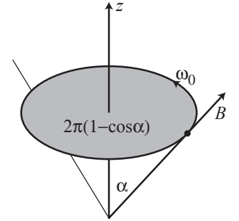
Fig. 14.17 The magnetic field vector revolves around the z -axis at constant angular velocity \omega_0 while the angle \alpha remains constant. By its motion it spans a solid angle 2\pi(1 - \cos \alpha) .
