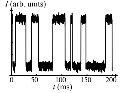
Fig. 18.5 Current through a detector quantum point contact switching in time as a result of charging and discharging of a nearby quantum dot with a single electron.
