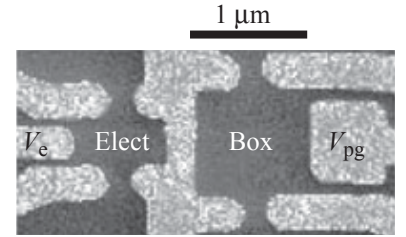
Fig. 18.6 Scanning electron micrograph of a circuit in which one quantum dot (Elect) is employed as a charge detector for the charge state of the neighboring quantum dot (Box). The structure is realized on a two-dimensional electron gas, bright regions represent metallic electrodes on the sample surface. (Reprinted with permission from Duncan et al. , 1999. Copyright 1999, American Institute of Physics.)
