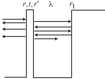
Fig. 21.2 Schematic illustration showing a square potential minimum coupled to a continuum of states to the left via a thin tunneling barrier with reflection coefficients r and r' , and transmission coefficient t . Propagation within the potential well leads to phase accumulation described by \lambda . At the potential step to the right, particles are totally reflected as described by the reflection amplitude r_t .
