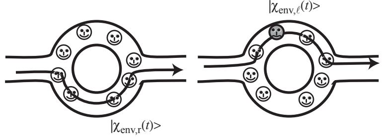
Fig. 14.23 Illustration of decoherence. The environment is represented by the smileys. Depending on the path of the electrons the resulting state of the environment differs. The environment measures the path of the electron and the interference disappears.
