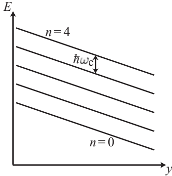
Fig. 16.6 Real space representation of the Landau level spectrum in the presence of an electric field in the y -direction. The slope of the Landau levels is given by -eE , and their spacing is \hbar\omega_c .
