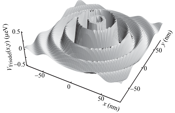
Fig. 9.10 Friedel oscillations in the plane. Parameters as for Fig. 9.9.
