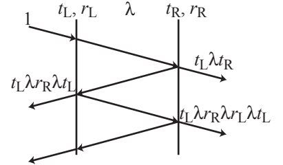
Fig. 18.28 Schematic of interfering paths reflected back and forth between two semitransparent mirrors, which are in quantum dot physics replaced by the tunneling barriers coupling the dot to source and drain.
