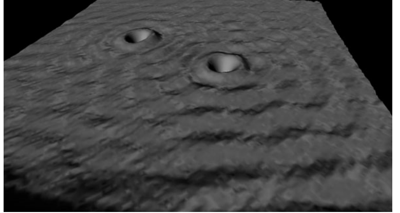
Fig. 9.11 Standing waves observed on a Cu(111) surface as observed with scanning tunneling microscope spectroscopy. Two point defects on the surface cause Friedel oscillations in the electron density that have here been mapped with real space and energy resolution (Crommie et al. , 1993).
