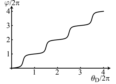
Fig. 21.3 Phase \varphi of the reflection coefficient of a cavity as a function of the round trip phase \theta_D within the cavity, assuming \alpha = 0 .
