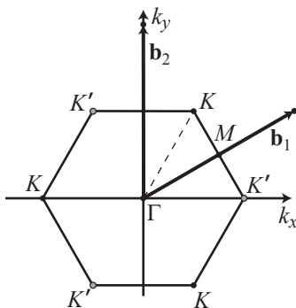
Fig. 3.6 First Brillouin zone of graphene with symmetry points \Gamma , \mathbf{K} , \mathbf{K}' , and \mathbf{M} , and the reciprocal lattice vectors \mathbf{b}_1 and \mathbf{b}_2 .
