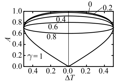
Fig. 21.14 Decoherence factor A as a function of \Delta\mathcal{T} for \mathcal{T} = 1/2 and a number of values for \gamma .
