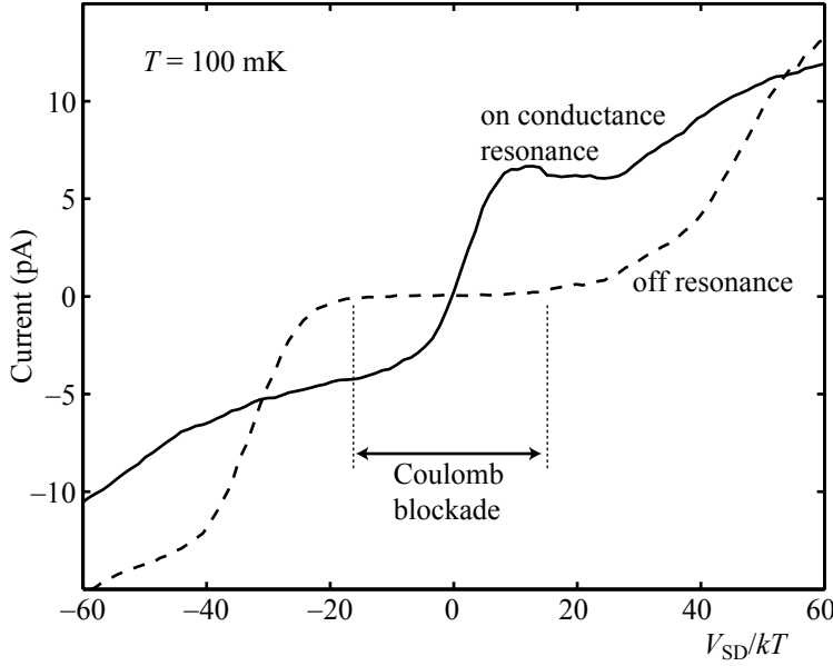
Fig. 18.2 Measured I(V_{SD}) trace of a quantum dot on a conductance resonance (solid line) and off resonance (dashed line). In the latter case the current is suppressed at low V_{SD} (Coulomb blockade).
