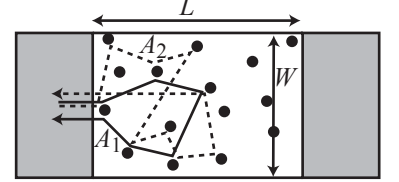
Fig. 14.27 Schematic sketch of a strongly disordered sample of width W and length L . Two specific paths contributing to the reflection probability with probability amplitudes A_1 and A_2 are shown as solid and dashed lines. They differ in their scattering sequences.
