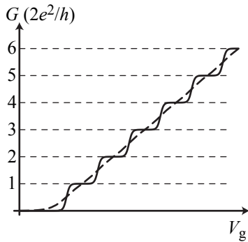
Fig. 11.4 Conductance as a function of gate voltage V_g according to eq. (11.8), assuming that the mode energies shift down proportional to the gate voltage. The spin degeneracy has been assumed to be g_s = 2 . If the temperature is significantly lower than the spacing between the mode energies, the conductance is quantized (solid line). If 4k_B T is comparable to the mode's energy spacing, the quantization is smoothed out (dashed curve).
