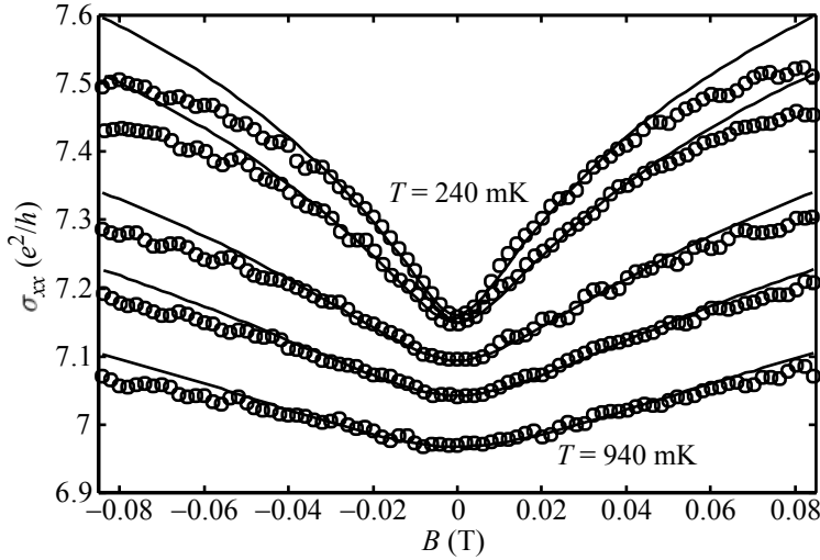
Fig. 15.6 Fit of the weak localization correction formula (15.6) to the measured data at different temperatures. From these fits, the phase coherence time \tau_\varphi can be determined. (Reprinted with permission from Senz et al. , 2000 b . Copyright 2000 by the American Physical Society.)
