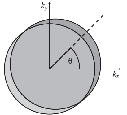
Fig. 10.17 Distribution function in k -space at finite electric and magnetic field. The distribution function is shifted from its equilibrium position by the amount \delta k = e\tau_0 \cos\theta |\mathbf{E}|/\hbar . The direction of the shift is given by the Hall angle \theta for which \tan\theta = \omega_c\tau .
