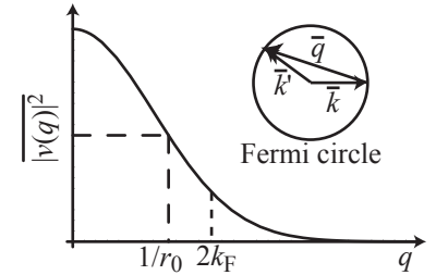
Fig. 10.23 The squared modulus of a typical scattering matrix element. At the top right, scattering vectors for a particular scattering process are shown. The maximum possible value for q is 2k_F .
