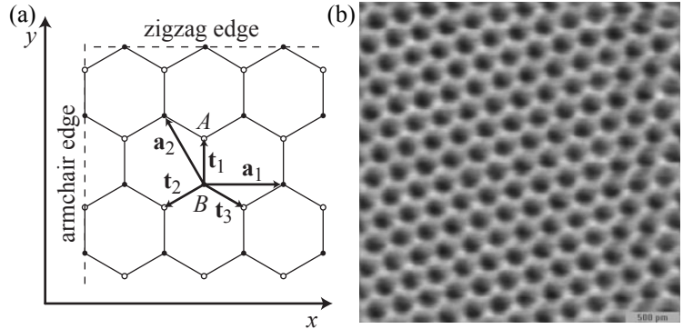
Fig. 3.5 (a) Graphene has a hexagonal lattice with a two-atom basis (atoms A and B). Lattice vectors are \mathbf{a}_1 and \mathbf{a}_2 . Characteristic edges are also indicated. The armchair edge has A and B atoms, whereas the zigzag edge has only one type of atom (A or B). (b) Scanning tunneling microscopy image of the graphene lattice with atomic resolution showing the hexagonal lattice structure (Li, 2003. Image courtesy of Eva Andrei, Rutgers University).
