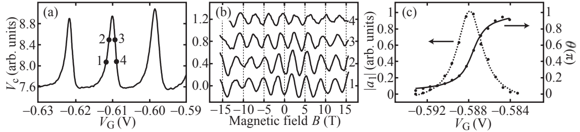
Fig. 21.11 (a) Collector voltage V_C measured as a function of the plunger gate voltage V_G of the quantum dot. (b) Aharonov–Bohm oscillations of V_C measured as a function of magnetic field. The Aharonov–Bohm period is indicated by vertical dashed lines. (c) Amplitude and phase extracted for one particular resonance. (Schuster et al. , 1997. Reprinted by permission from Macmillan Publishers Ltd, copyright 1997.)
