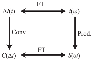
Fig. 20.1 Functions used to characterize electronic noise, and the relation between them.
