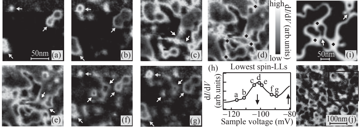
Fig. 16.26 Local density of states measured in the lowest spin-resolved Landau level of an InSb two-dimensional electron gas by scanning tunneling spectroscopy at a magnetic field B = 12 T. See text for details. (Reprinted with permission from Hashimoto et al. , 2008. Copyright 2008 by the American Physical Society.)
