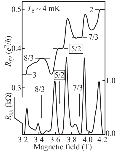
Fig. 16.35 Measurement of the fractional structure of the third Landau level around filling factor \nu = 5/2 in a GaAs/AlGaAs heterostructure at the temperature T = 4 mK. (Reprinted with permission from Pan et al. , 1999. Copyright 1999 by the American Physical Society.)
