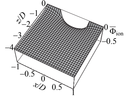
Fig. 7.5 Normalized potential of the donor layer \Phi_{\text{ion}}(x, z) .
