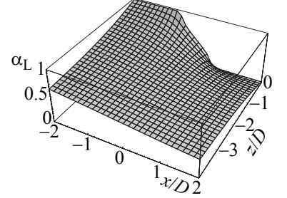
Fig. 7.4 Characteristic potential of the left gate, \alpha_L(x, z) .
