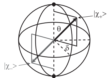
Fig. 3.9 Bloch sphere representation of the electron spin.
