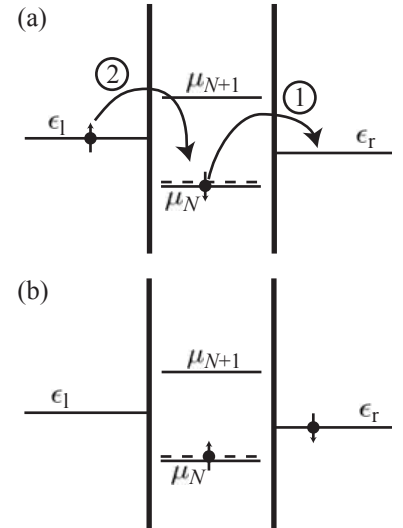
Fig. 18.42 Lowest order cotunneling process contributing to the Kondo effect. (a) Initial state and cotunneling processes. (b) Final state after the correlated tunneling event.
