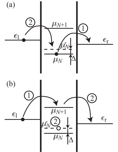
Fig. 18.39 Two processes contributing to inelastic cotunneling.
