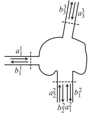
Fig. 13.2 Incoming probability amplitudes a_n^\alpha impinging onto a mesoscopic system and outgoing amplitudes b_n^\alpha . The index \alpha labels a particular lead, n numbers a particular mode in lead \alpha .
