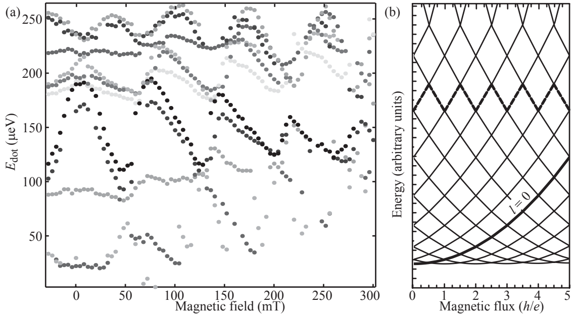
Fig. 18.22 (a) Measured magnetic field dispersion of the conductance resonances in a quantum ring. A constant charging energy of 190\text{ }\mu\text{eV} has been subtracted between neighboring states. (b) Calculated spectrum of an ideal one-dimensional quantum ring (Fuhrer et al. , 2001).
