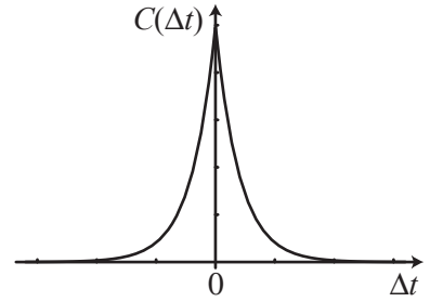
Fig. 20.2 Exponential decay of the autocorrelation function C(\Delta t) .
