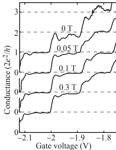
Fig. 11.13 Conductance of a quantum point contact showing the suppression of transmission resonances by a magnetic field. (Reprinted with permission from van Wees et al. , 1991. Copyright 1991 by the American Physical Society.)
