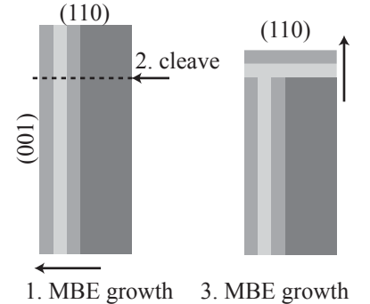
Fig. 6.3 Schematic presentation of the cleaved-edge overgrowth (CEO) method.
