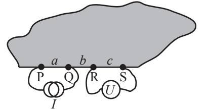
Fig. 10.14 Arrangement of four contacts along the edge of an electron gas filling a semi-infinite plane.
