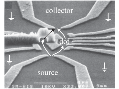
Fig. 21.9 Scanning electron micrograph of the sample used for the transmission phase measurement. A voltage is applied between the source contact and ground. The voltage between the collector contact and ground is measured. (Schuster et al. , 1997. Reprinted by permission from Macmillan Publishers Ltd, copyright 1997.)
